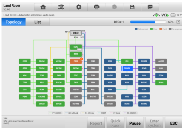
Figure 4-8 Topology Screen
