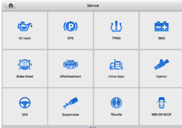
Figure 5-1 Service Menu
