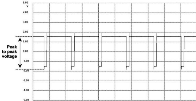
Figure 18-2 Square Waveform
