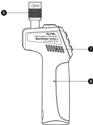
Figure 2-5 MaxiVideo MV500-2 Handle Left Side View
