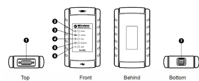
Figure 2-5 Wireless Diagnostic Interface
