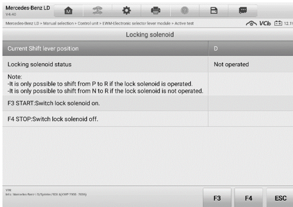
Figure 4-15 Sample Active Test Screen
