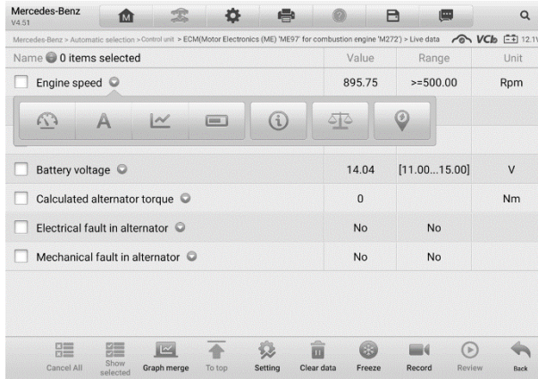
Figure 4-11 Sample Display Mode Screen
