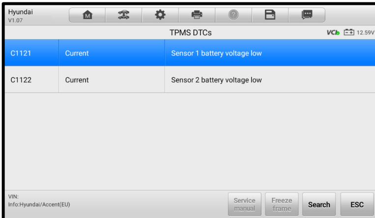
Figure 6-12 DTCs Screen
