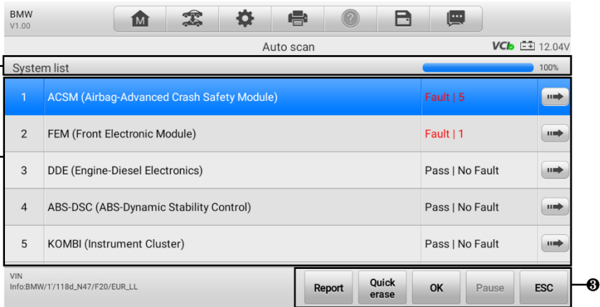
Figure 4-9 Auto Scan Screen
