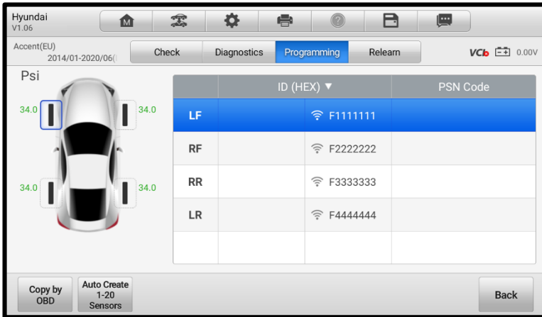
Figure 6-25 Programming Screen 2
