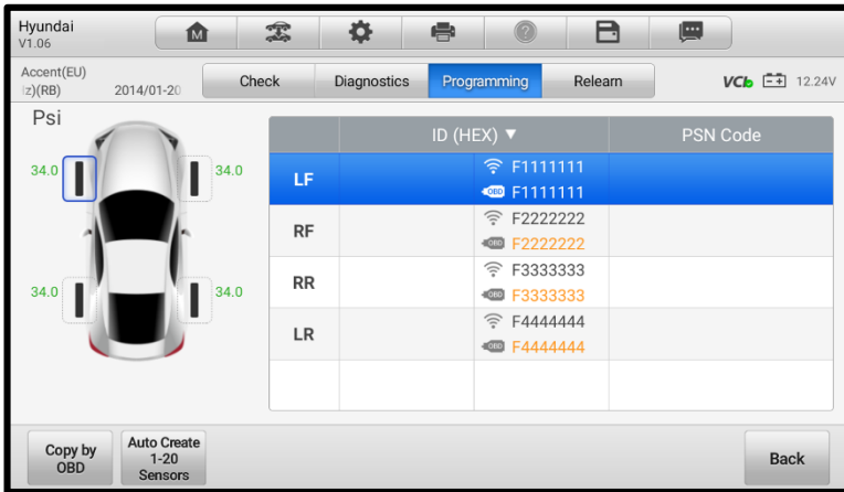
Figure 6-24 Programming Screen 1
