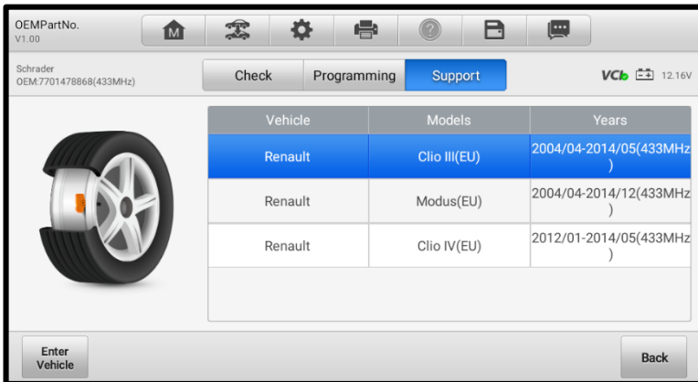
Figure 6-41 Support Screen
