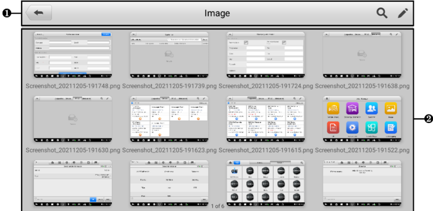
Figure 11-5 Image Screen
