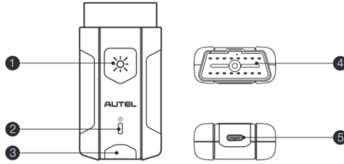
Figure 2-5 MaxiVCI V200 Views
