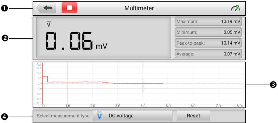
Figure 11-5 Multimeter Screen
