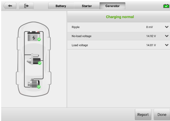
Figure 6-6 Generator Test Results Screen
