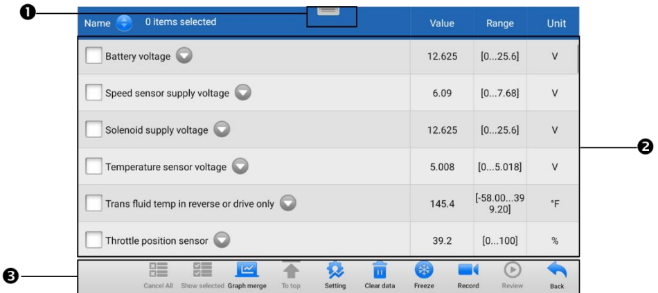
Figure 9-11 Live Data Screen
