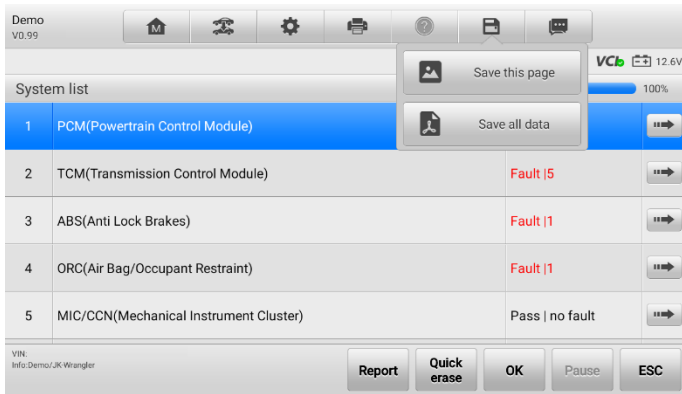
Figure 9-18 Auto Scan Screen
