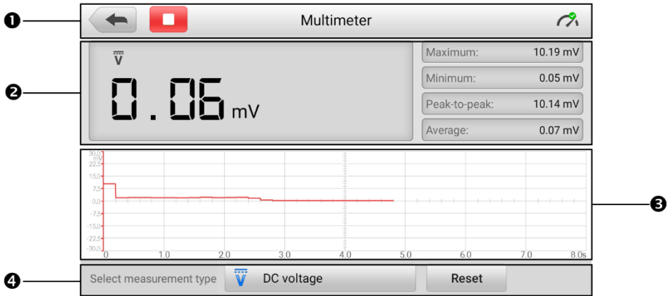
Figure 11-5 Multimeter Screen
