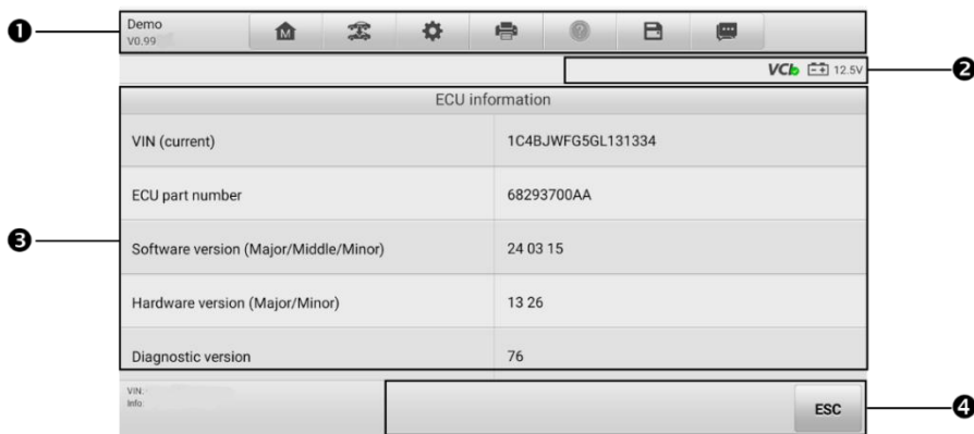
Figure 9-9 ECU Information Screen
