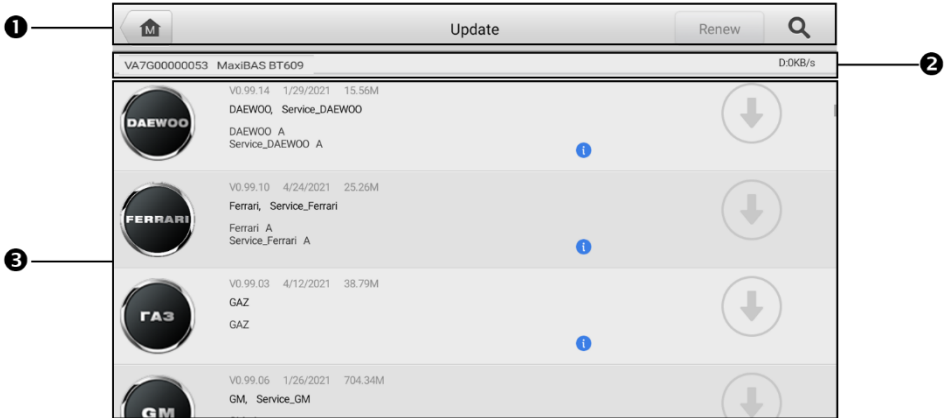
Figure 13-1 Update Screen
