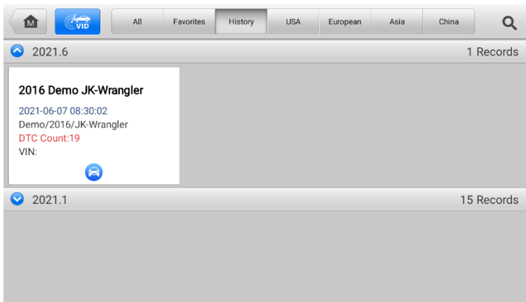
Figure 9-17 History Screen
