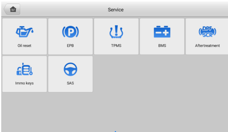
Figure 10-1 Service Menu
