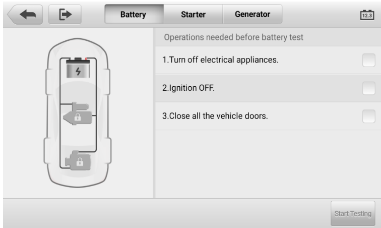
Figure 4-4 Battery Screen
