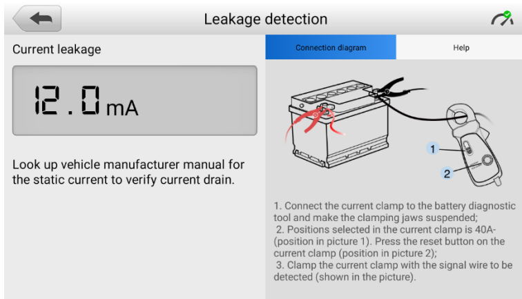
Figure 11-2 Leakage Detection (Current Model) Screen
