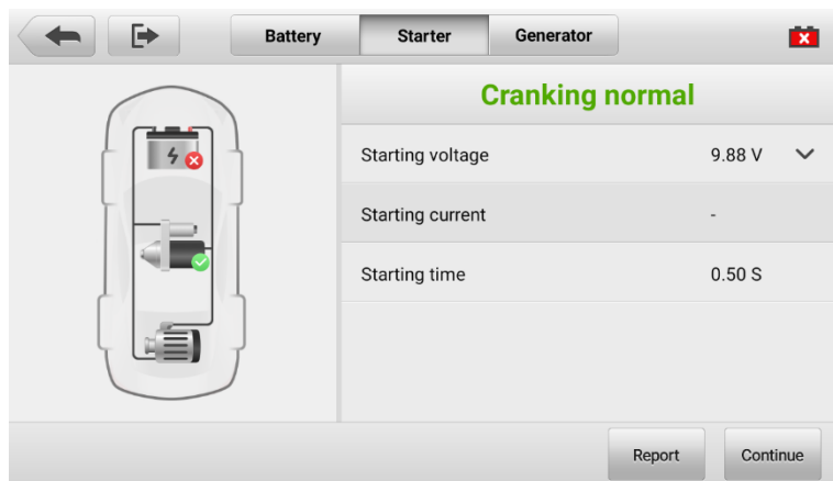
Figure 4-6 Starter Test Result Screen
