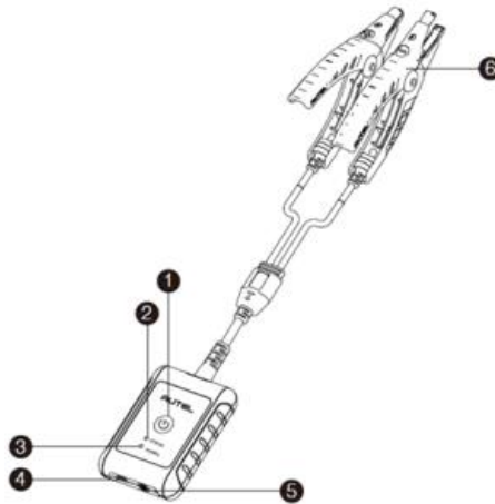
Figure 2-4 MaxiBAS B200 View
