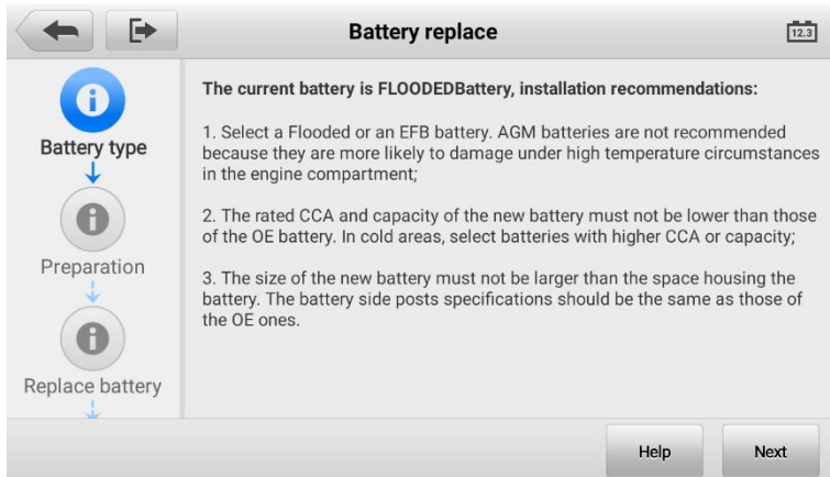
Figure 6-1 Battery Replace Screen
