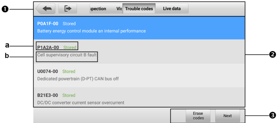
Figure 8-3 Trouble Codes Screen
