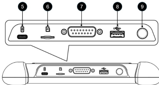
Figure 2-2 Tablet Top View
