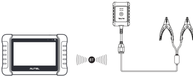
Figure 13-3 Battery Tester Connection Example 1
