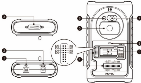
Figure 2-5 XP400 Pro Views
