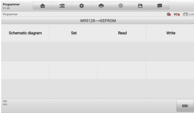
Figure 5-4 Read Menu
