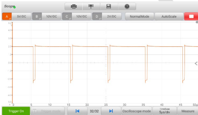
Figure 18-2 Square Waveform Screen
