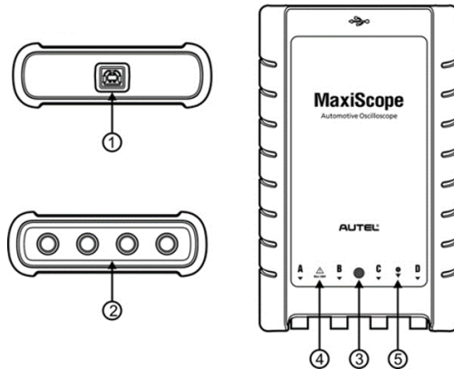
Figure 18-3 MaxiScope Module
