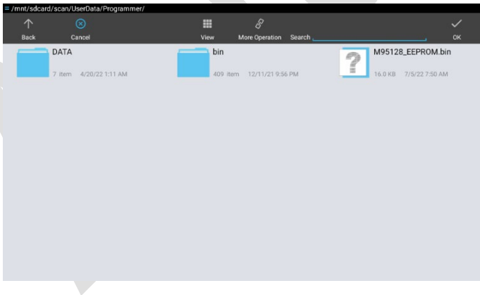
Figure 5-7 Write Screen
