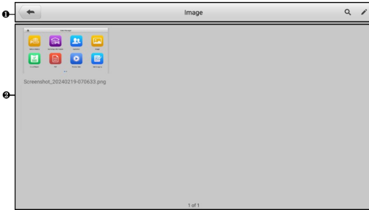
Figure 11-4 Image Screen
