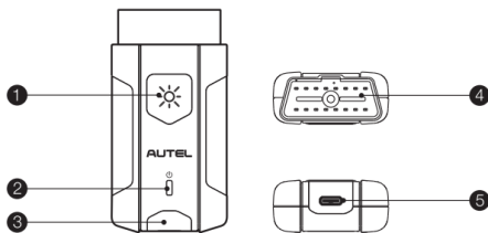
Figure 2-3 MaxiVCI V200 Views
